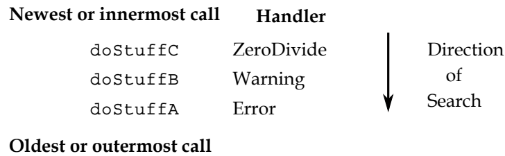
Figure 14.3 Selecting a Handler
