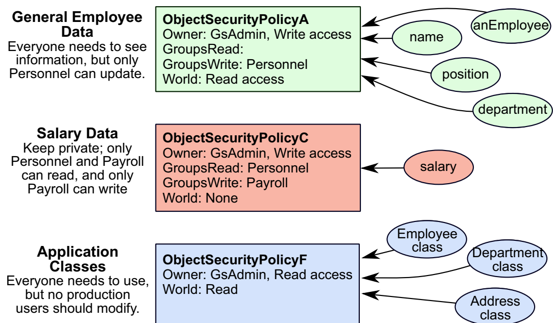
Figure 9.3 Application Objects Assigned with Three Security Policies
