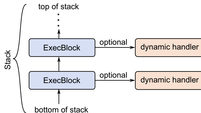
Figure 14.2 ExecBlock and Associated Handlers
