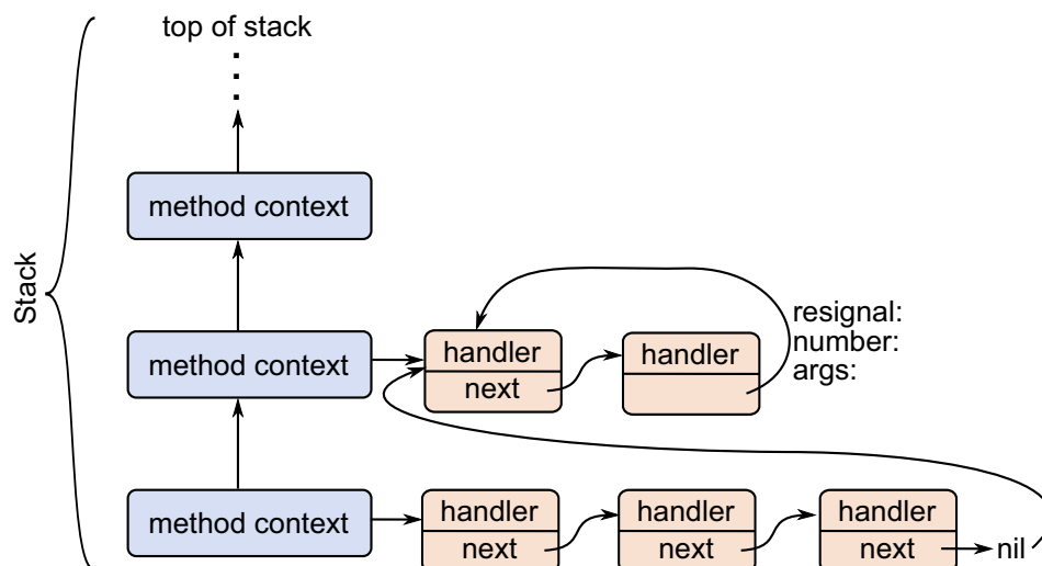
Figure 14.4 Method Contexts and Associated Handlers
