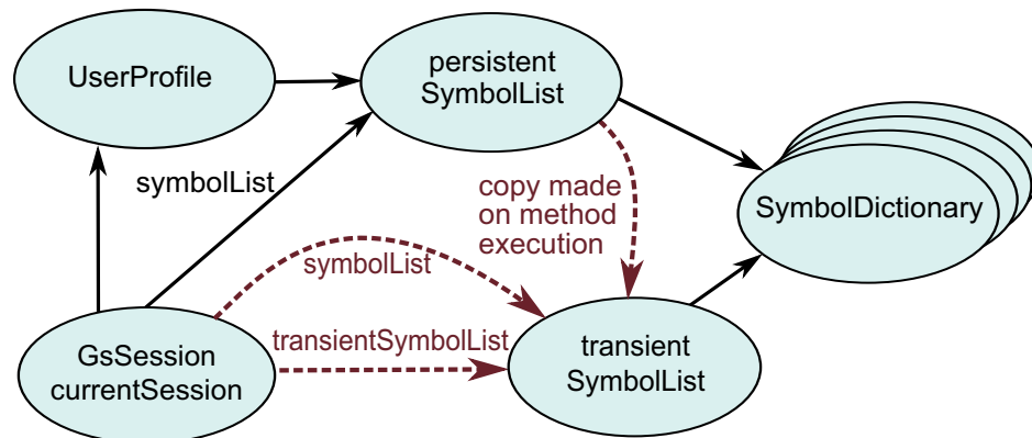
Figure 3.2 The GsSession symbolList – a copy of the UserProfile symbolList
