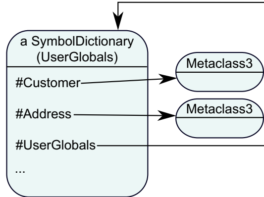
Figure 3.1 Self-Referencing Symbol Dictionary
