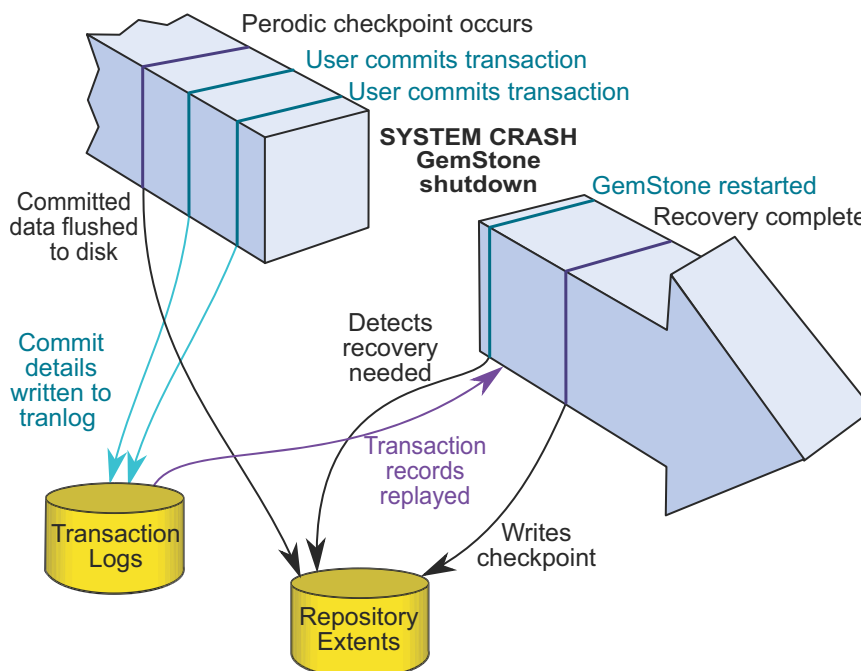
Figure 10.2 System Crash
