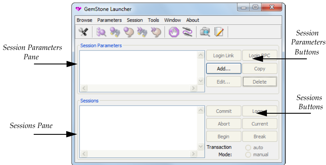
Figure 11.1 GemStone Launcher
