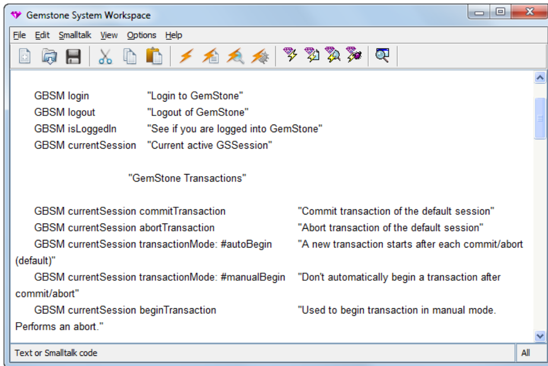
Figure 11.5 System Workspace
