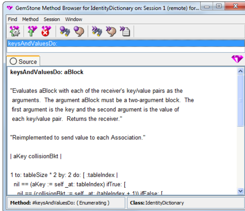
Figure 12.6 Method Browser
