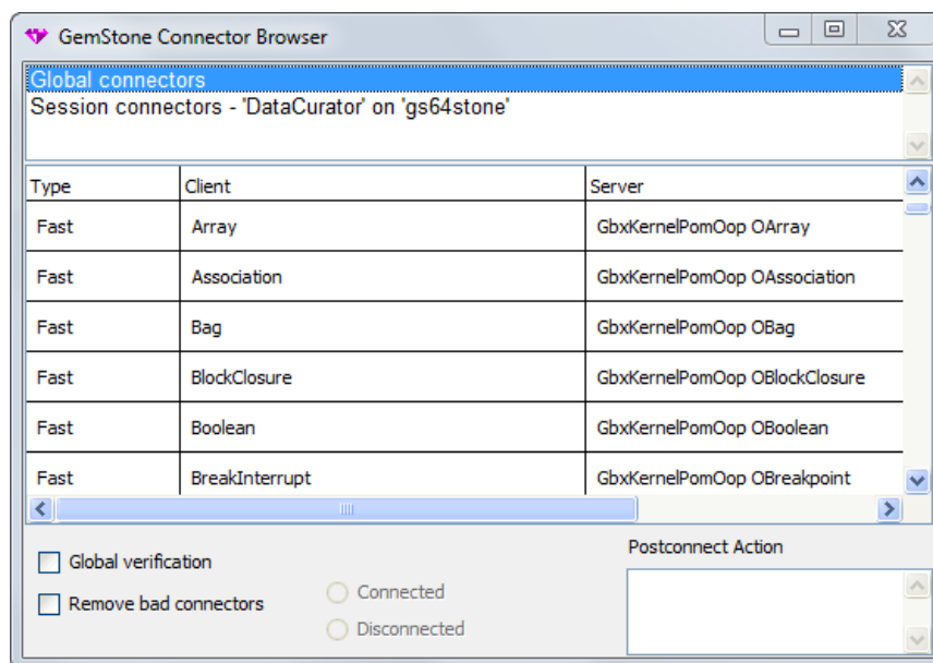
Figure 12.9 Connector Browser
