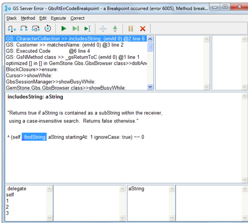
Figure 13.1 Debugger
