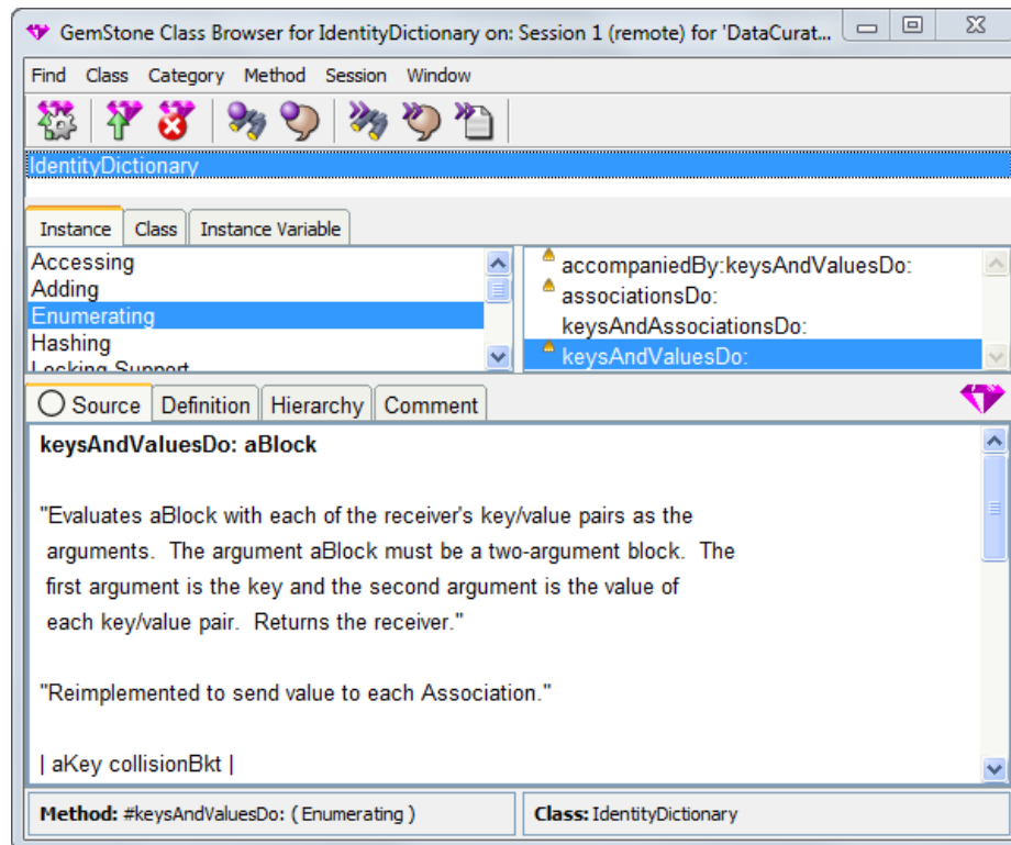
Figure 12.4 Class Browser
