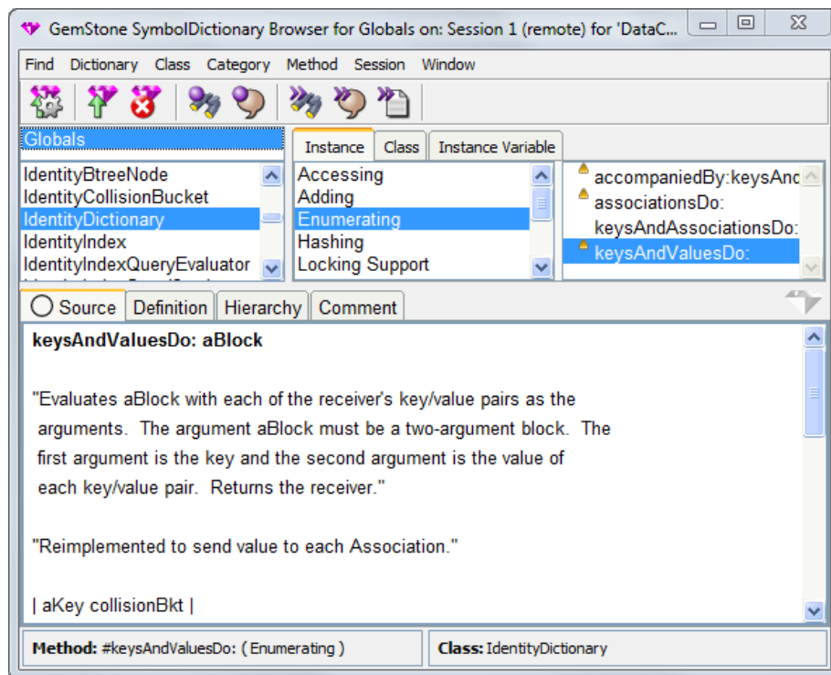
Figure 12.2 SymbolDictionary Browser
