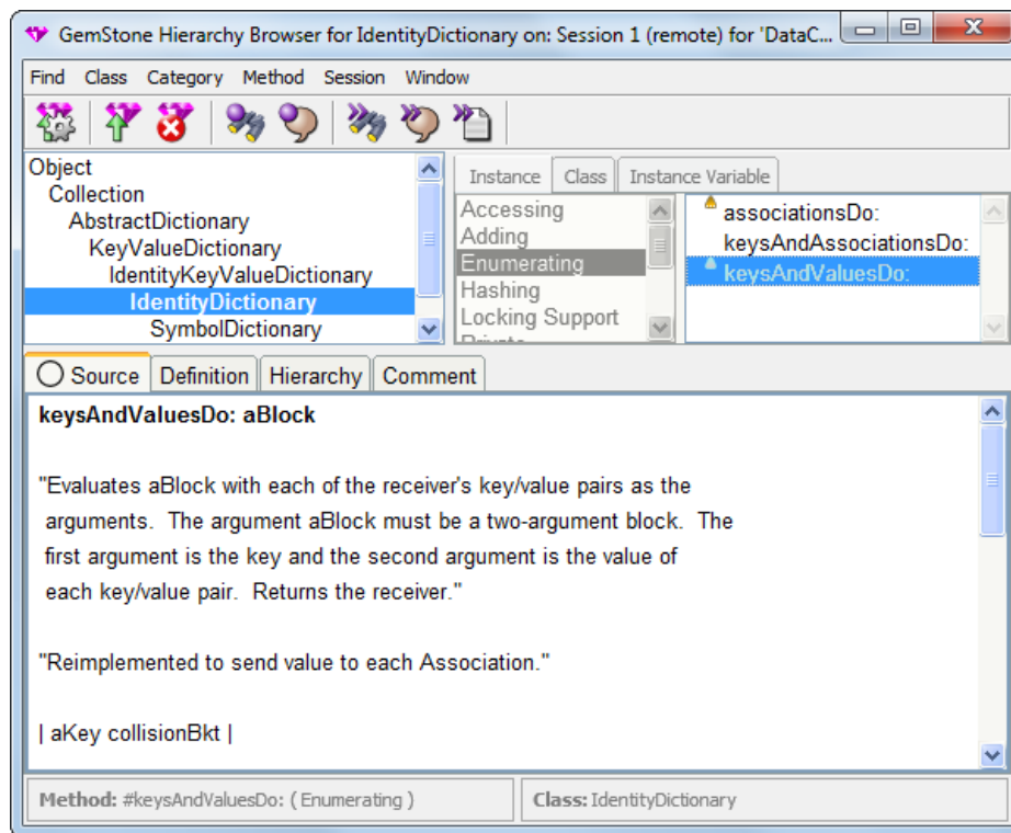
Figure 12.3 Hierarchy Browser
