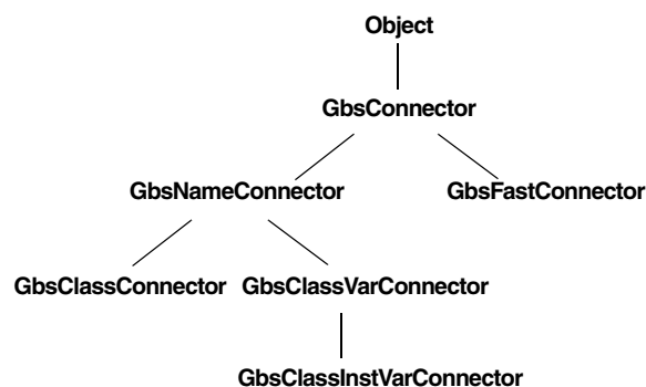
Figure 4.4 Connector Class Hierarchy
