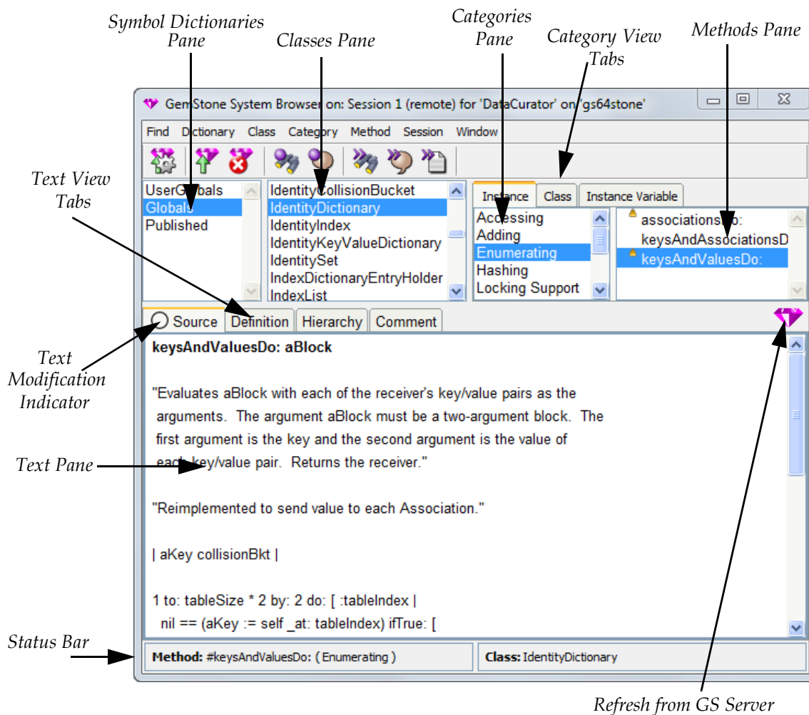
Figure 12.1 GemStone System Browser
