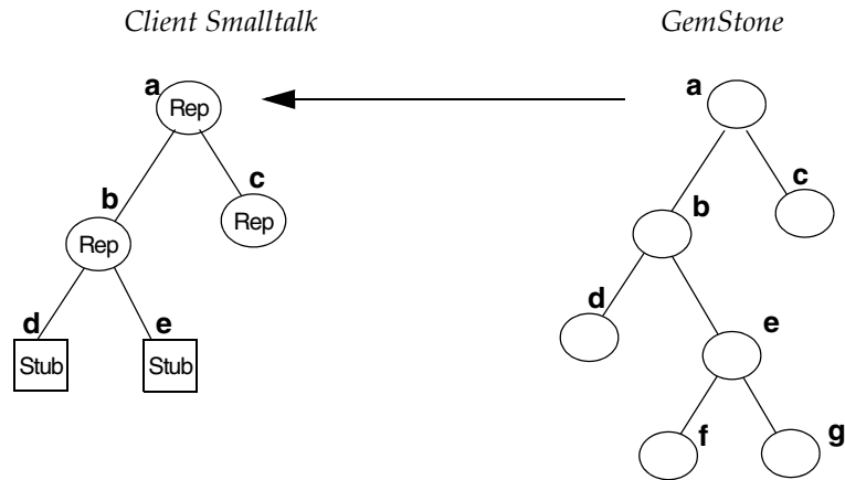
Figure 3.1 Two-level Fault of an Object
