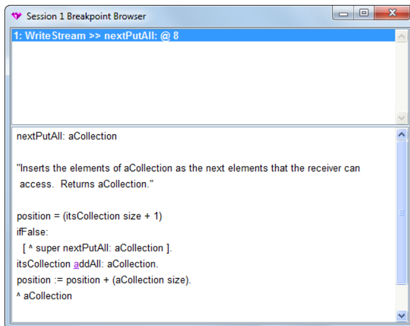
Figure 13.2 Breakpoint Browser
