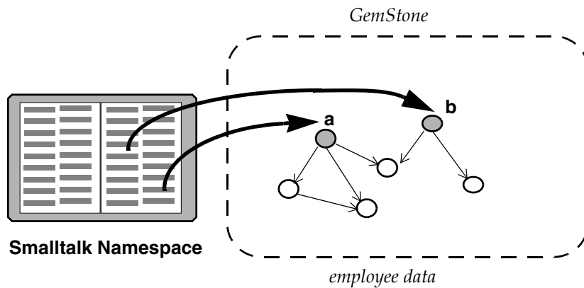
Figure 4.2 Root Objects
