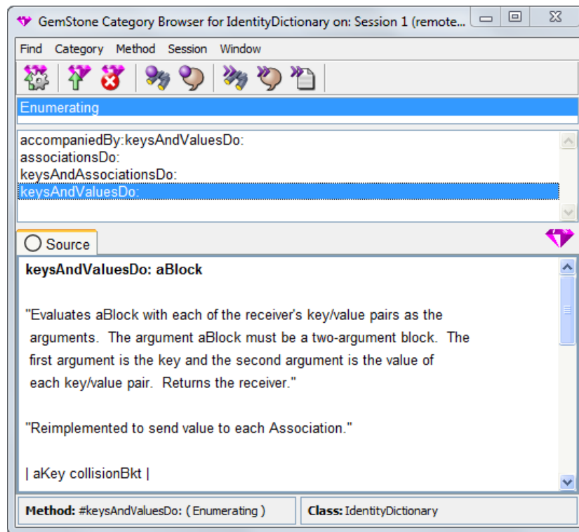
Figure 12.5 Category Browser
