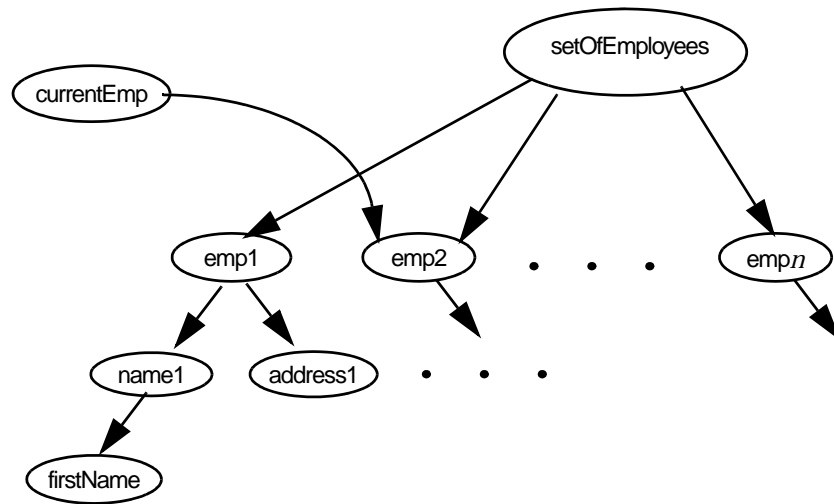
Figure 9.1 Employee Set Faulted into the Client Smalltalk
