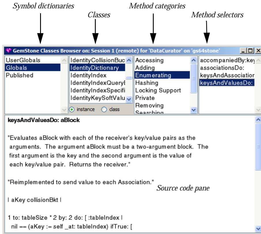
Figure 12.1 GemStone Classes Browser
