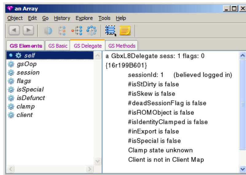
Figure 12.5 GemStone Inspector GS Delegate tab
