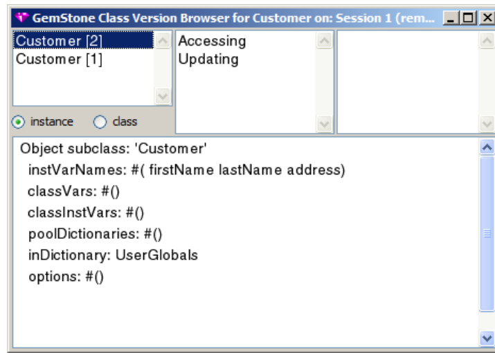
Figure 12.3 The Class Version Browser
