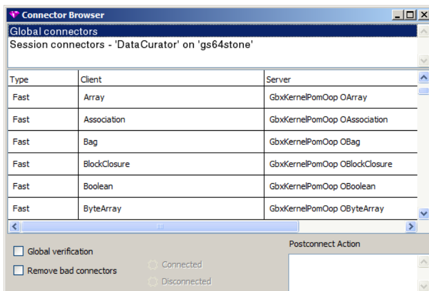
Figure 12.2 The Connector Browser
