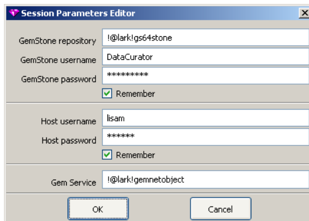
Figure 11.2 The Session Parameters Editor
