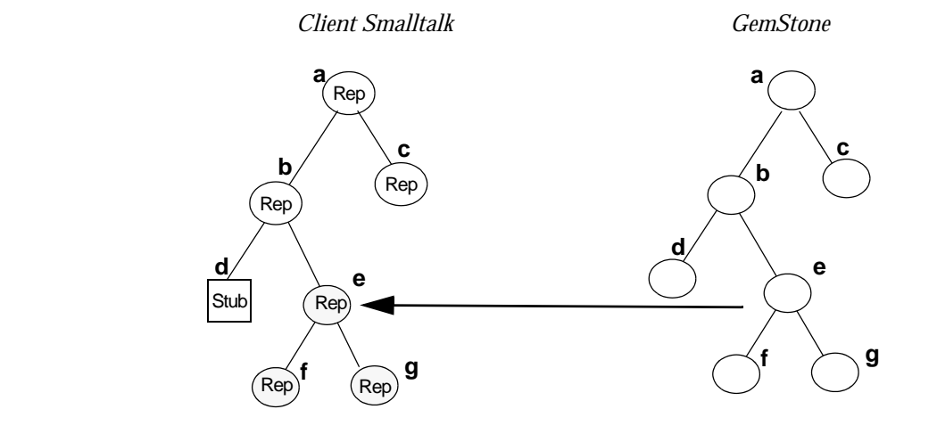
Figure 3.2 A Stub Responds to a Message
