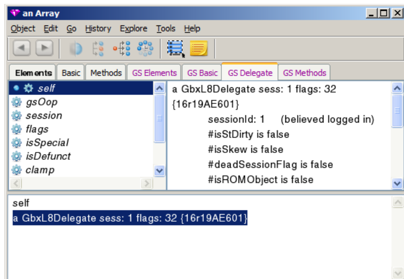
Figure 12.7 Evaluating “self” in the GS Delegate tab of the Inspector
