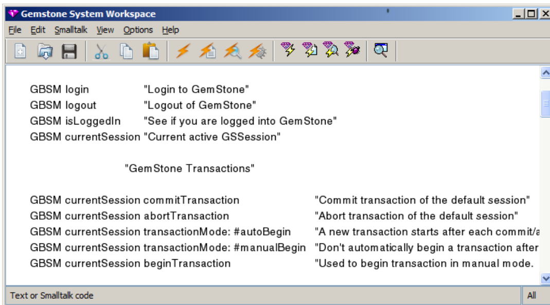
Figure 11.5 GemStone System Workspace
