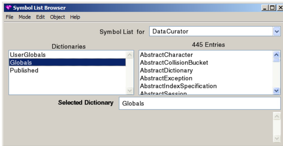
Figure 13.2 The Symbol List Browser
