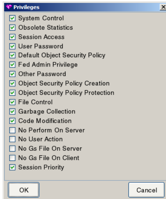
Figure 13.5 Privileges Dialog in GemStone User Window
