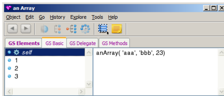
Figure 12.4 GemStone inspector
