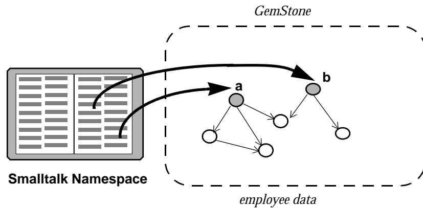
Figure 4.2 Root Objects
