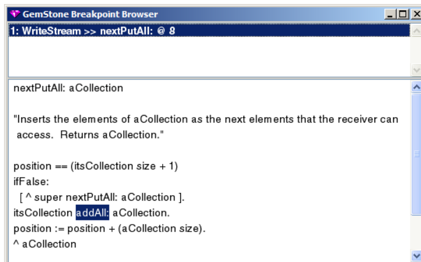
Figure 12.8 GemStone Breakpoint Browser with a Breakpoint
